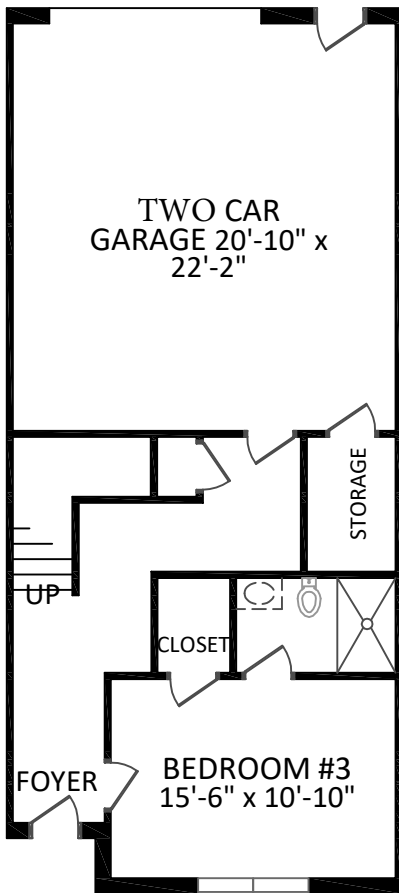
1ST FLOOR
